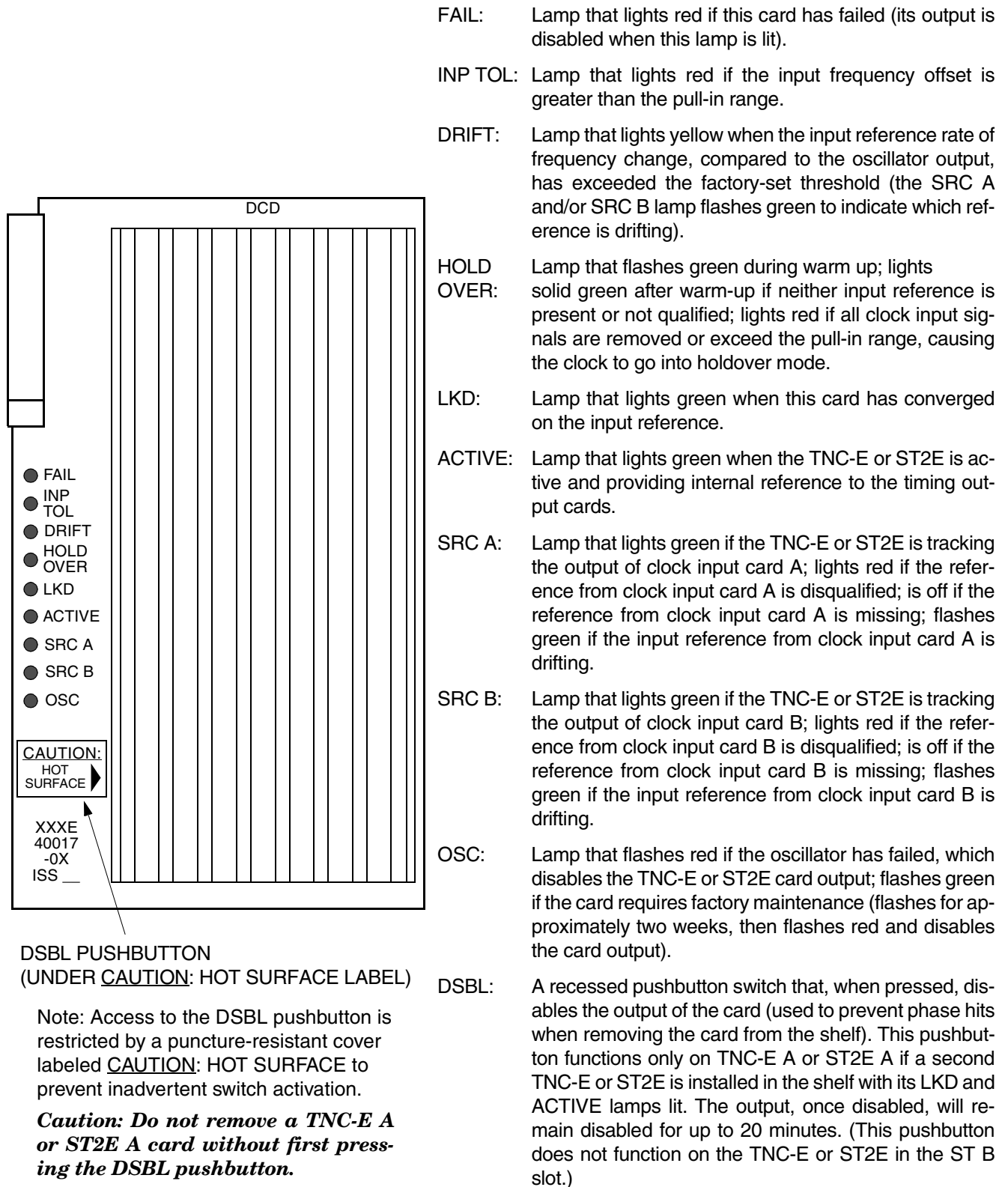
Figure 10. TNC-E and ST2E Card Controls and Indicators
